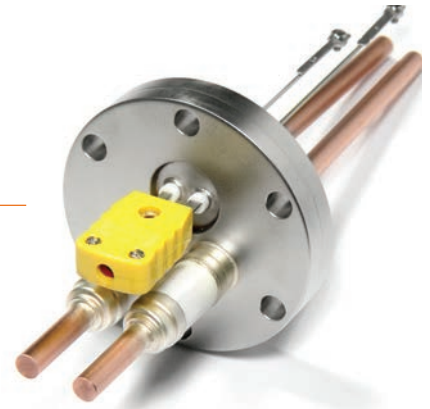
DN40CF Thermocouple type K with 2 x power pins
