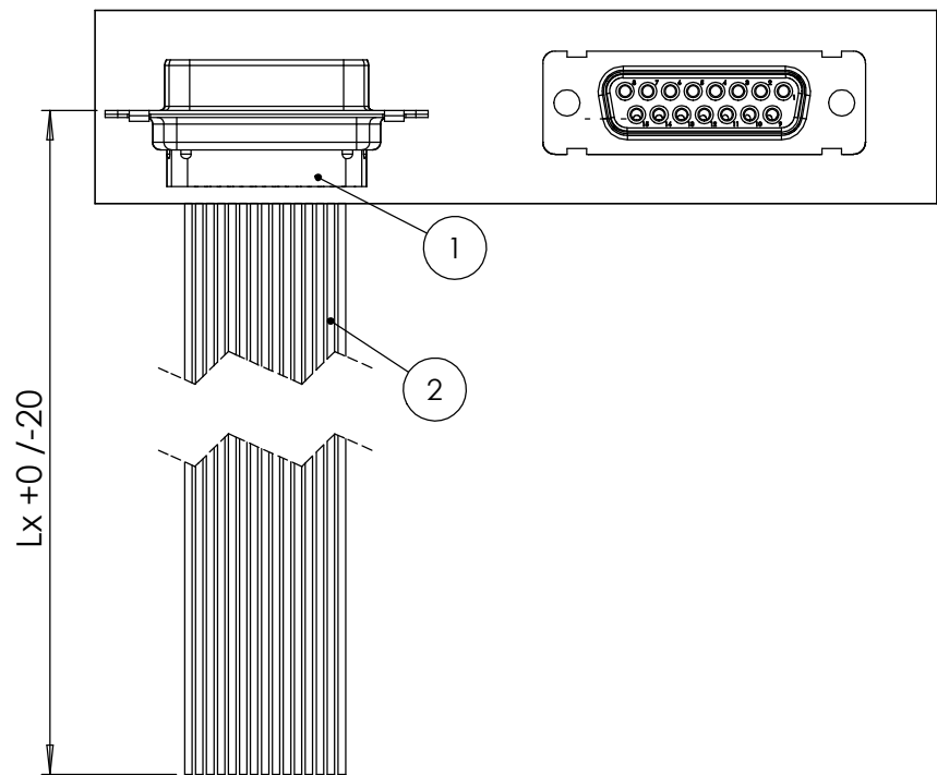
Connector 1/ 211-FS15-HV basic for feedthrough
