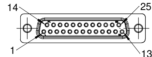
connector 2 / 211-FS25-HV-V2 basic customer 01
