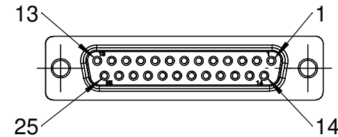
connector 1 / 211-FS25-HV-V2 basic for feedthrough 01
