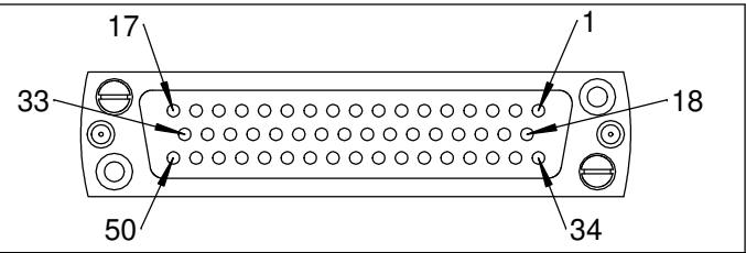
connector 1 / 211-FS50-PK basic for feedthrough
