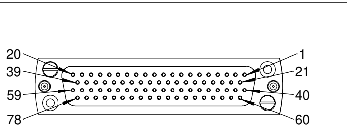
connector 1 / 211-FS78H-PK basic for feedthrough
